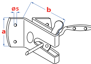
Gate latch automatic
